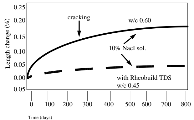
Fig. 5 - Effect of Rheobuild TDS on the alkali-aggregate reaction. Dosage of Portland cement: 350 \text{ kg/m}^3 ; slump: 200 mm; potentially reactive aggregates (max. size: 20mm)
