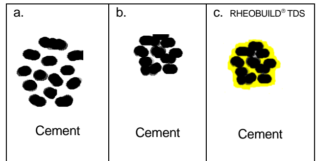
Fig. 1 - Schematic representation of cement paste in ordinary concrete (a), in concrete with superplasticizer (b) and in concrete with RHEOBUILD® TDS (c). Mix water is present among cement grains. Due to the superplasticizer, mix water is reduced, so that the distance among cement grains lowers. Consequently, the microstructure is denser and more compact (a → b). Besides the higher density deriving from the water reduction due to the presence of the superplasticizer, further increase in micro structural density occurs because of the filling of the interstitial voids among cement grains by amorphous silica particles, much smaller than cement grains (a → c).
