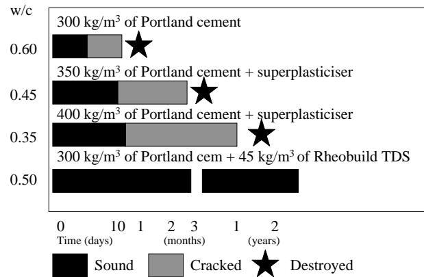
Fig 3 - The attack of 30% calcium chloride aqueous solution on concrete specimens kept at 5°C.
